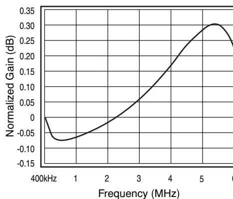
Figure 4. HD Flatness vs. Frequency
