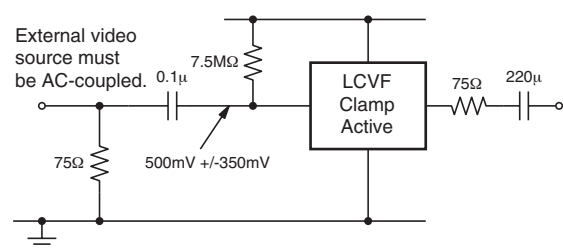
Figure 17. Biased SCART with AC-coupled Outputs
