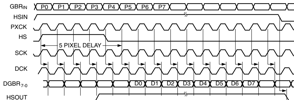
Figure 8. GBR Mode
