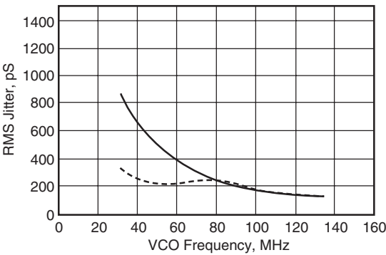
Figure 22. Pixel Clock RMS Jitter
