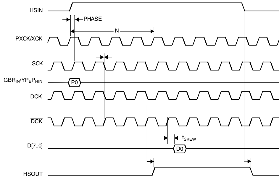
Figure 7. Output Timing
