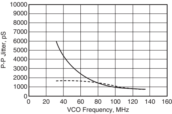
Figure 21. Pixel Clock Peak-to-Peak Jitter
