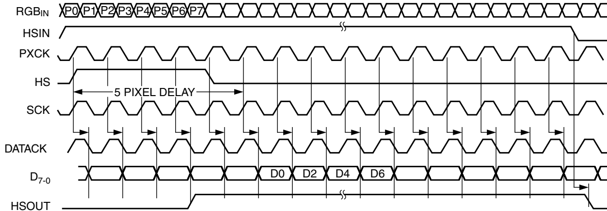
Figure 12. RGB Alternate Pixel Sampling Mode, (Odd Pixels)
