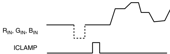
Figure 1. Clamping to the back-porch
