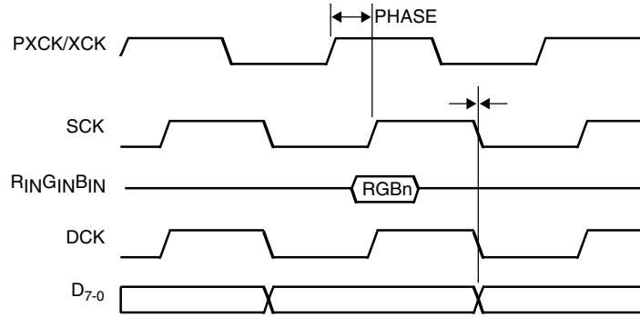
Figure 3. Internal Sampling Clock, SCK Timing
