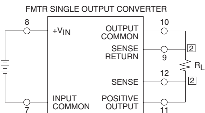
REMOTE SENSE CONNECTION 2 Make connections at load.
