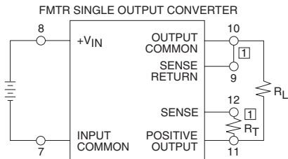
EXTERNAL TRIM CONNECTION 1 Make connections at converter.
