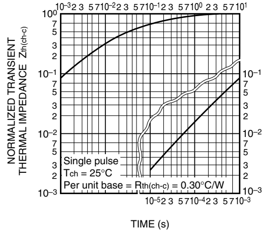
TRANSIENT THERMAL IMPEDANCE CHARACTERISTICS
