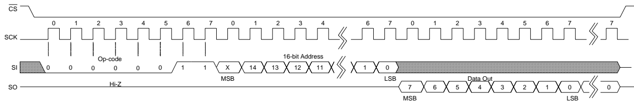
Figure 10. Memory Read
