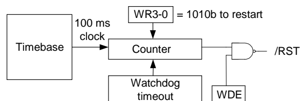
Figure 3. Watchdog Timer
