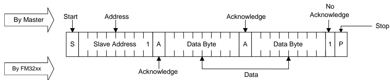
Figure 13. Sequential Memory Read
