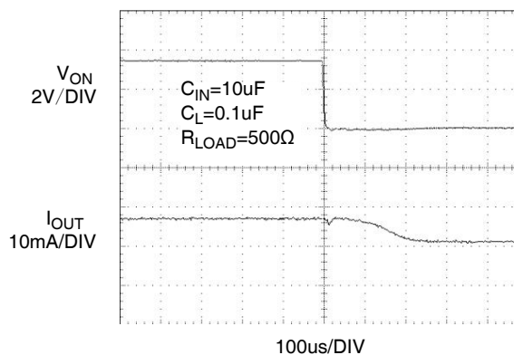
Figure 16. T_{OFF} Response
