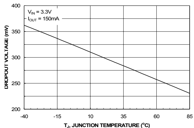
Figure 10. Drop Voltage vs. Temperature
