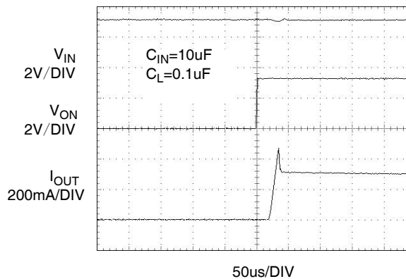
Figure 18. Current Limit Response Time (Output has a 4.7\Omega load)
