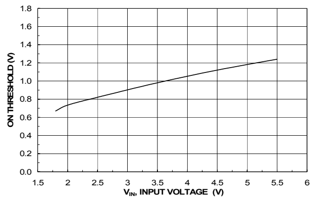
Figure 6. Input Voltage vs. On Threshold Voltage
