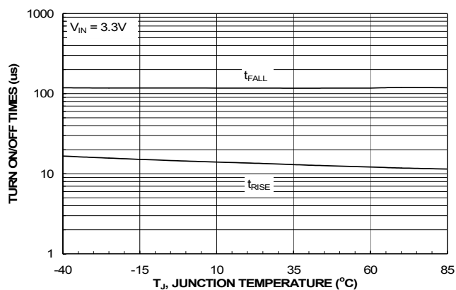
Figure 12. T RISE /T FALL vs. Temperature
