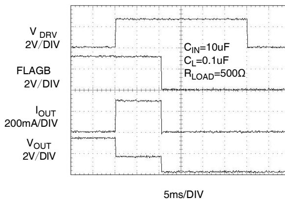
Figure 14. T_{BLANK} Response
