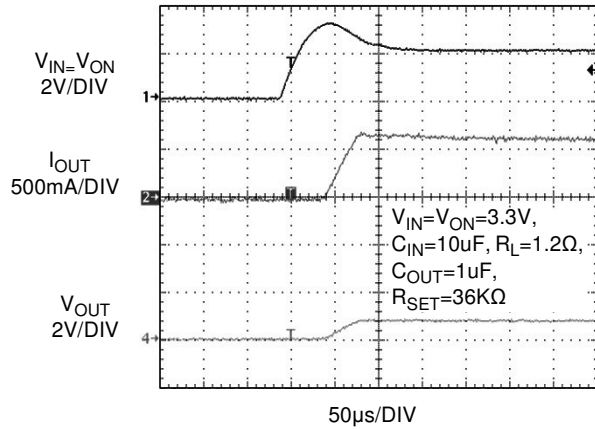
Figure 21. Current Limit Response (Switch is powered into a short - Input and enable pin are tied together)
