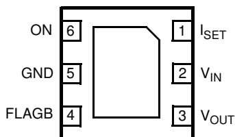
MicroFET 2x2 6L (BOTTOMVIEW)
