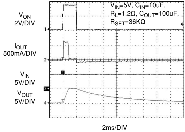
Figure 20. Current Limit and Output Discharge Response (Device turns on and off into large capacitive load C_{OUT}=100\text{F} )
