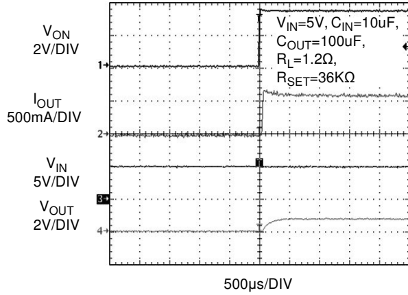
Figure 19. Current Limit Response (Output is loaded with 1.2Ω resistor and C_{OUT}=100\mu\text{F} )
