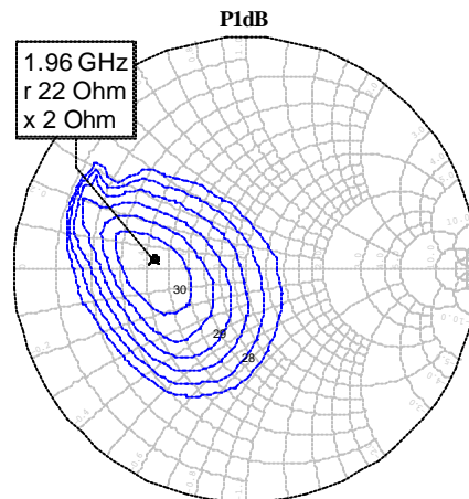
Maximum P1dB = +30.9 dBm at Z_L = 22 + j2\ \Omega
