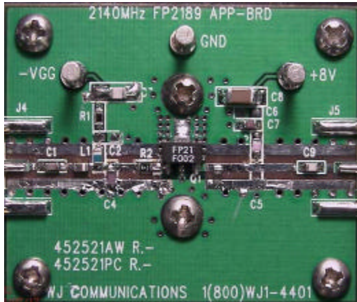
14 mil GETEK™ ML200DSS ( \epsilon_r = 4.2 ) The main microstrip line has a line impedance of 50 O.
