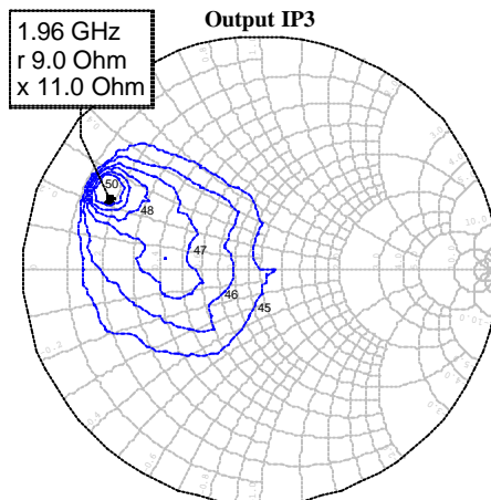
Maximum IP3 = +51 dBm at Z_L = 9 + j11\ \Omega
