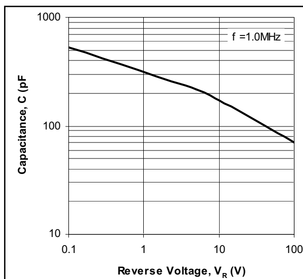
Figure 4. Typical Capacitance
