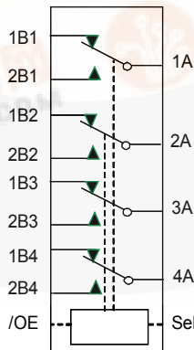
Figure 1. Analog Symbol
