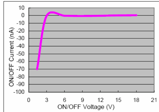
FSP3123 ON/OFF Current v.s. ON/OFF Voltage ( V_{in}=12V )
