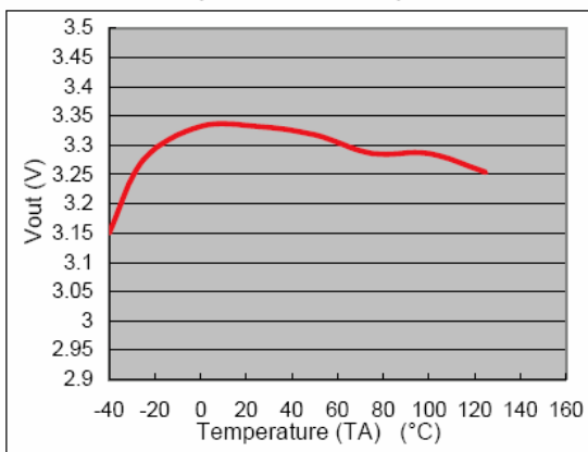
FSP3123 Output Voltage v.s. Temperature ( V_{in}=12V , I_o=3A )
