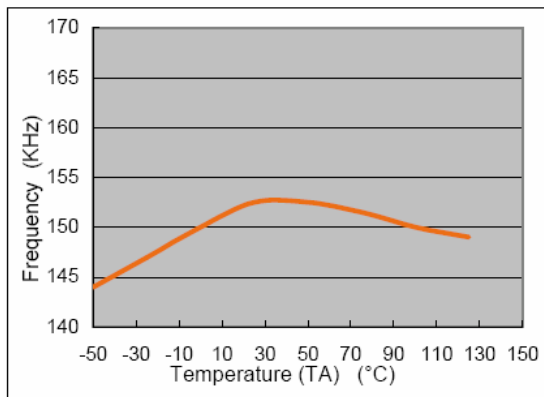
FSP3123 Frequency v.s. Temperature ( V_{CC}=12V , I_o=500mA , V_{out}=5V )
