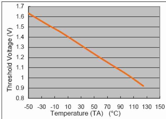
FSP3123 Threshold Voltage v.s. Temperature ( V_{CC}=12V , I_o=100mA )
