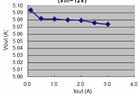
FSP3131 Load Regulation (Vin=12V)
