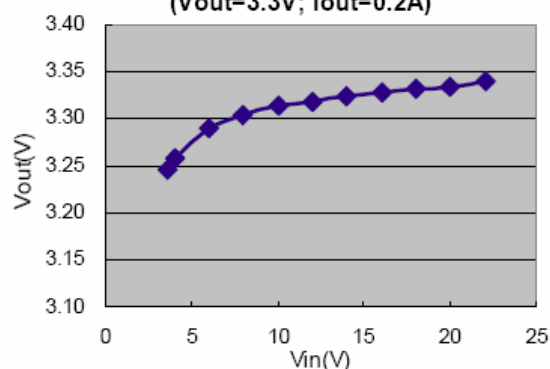
FSP3131 Line Regulation (Vout=3.3V; Iout=0.2A)
