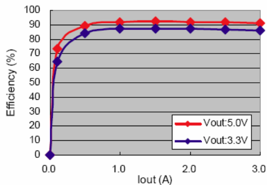
FSP3131 Efficiency
