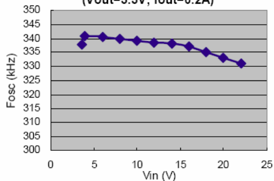
FSP3131 Vin vs. Frequency (Vout=3.3V; Iout=0.2A)
