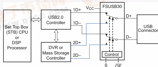
Figure 1. Typical Application
