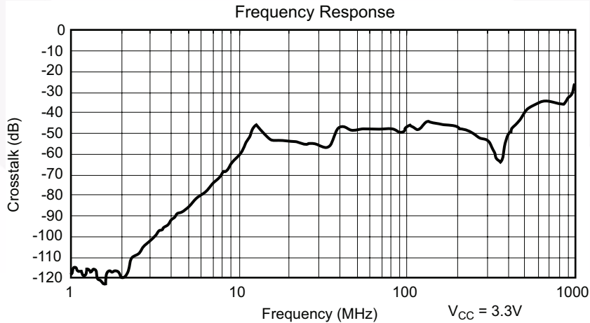
Figure 4. Crosstalk
