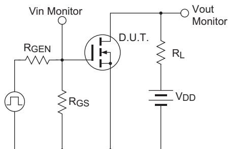
Switching Time Measurement Circuit
