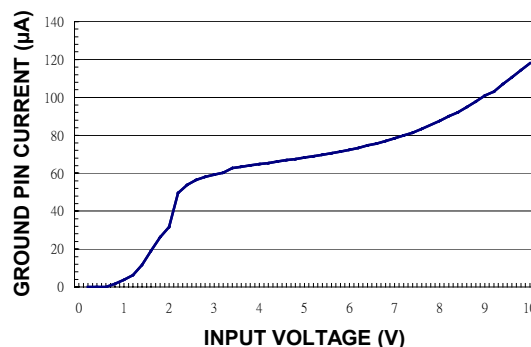
GROUND PIN CURRENT vs. INPUT VOLTAGE
