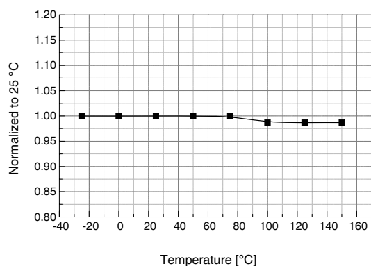
Figure 5. Start Threshold Voltage vs. Temp.
