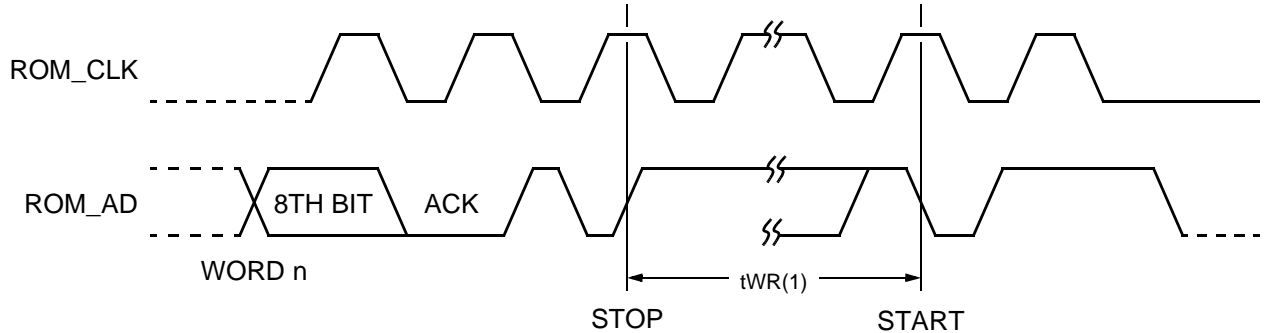
Figure 8. Bus Timing
