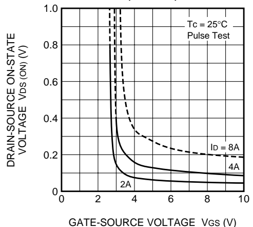
ON-STATE VOLTAGE VS. GATE-SOURCE VOLTAGE (TYPICAL)
