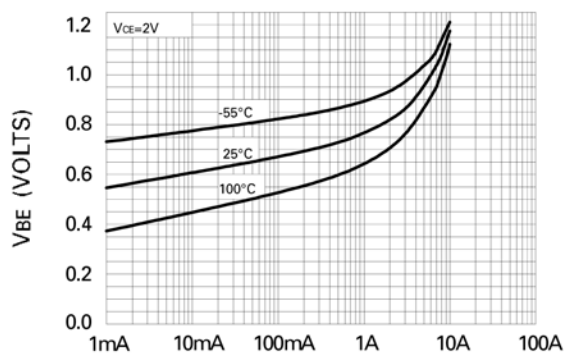
Collector Current
