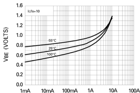
Collector Current
