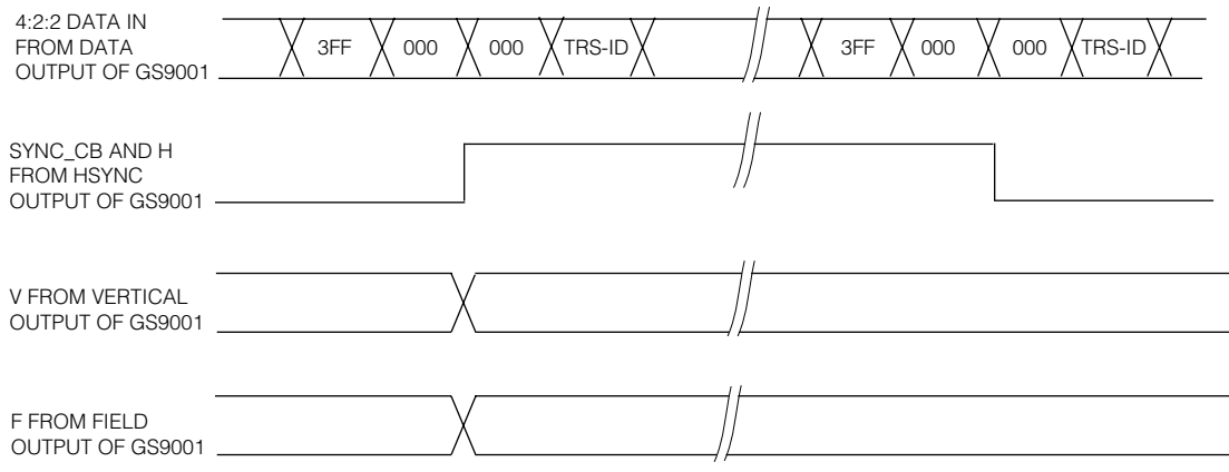
Fig. 9d Relative Timing of Data, SYNC_CB, H, V and F Inputs (GS9001 = 1)
