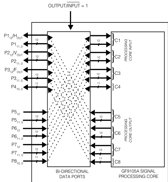
Fig. 4d Functional Block Diagram of GF9105A (OUTPUT/INPUT = 1, HVF_OUT = 1)
