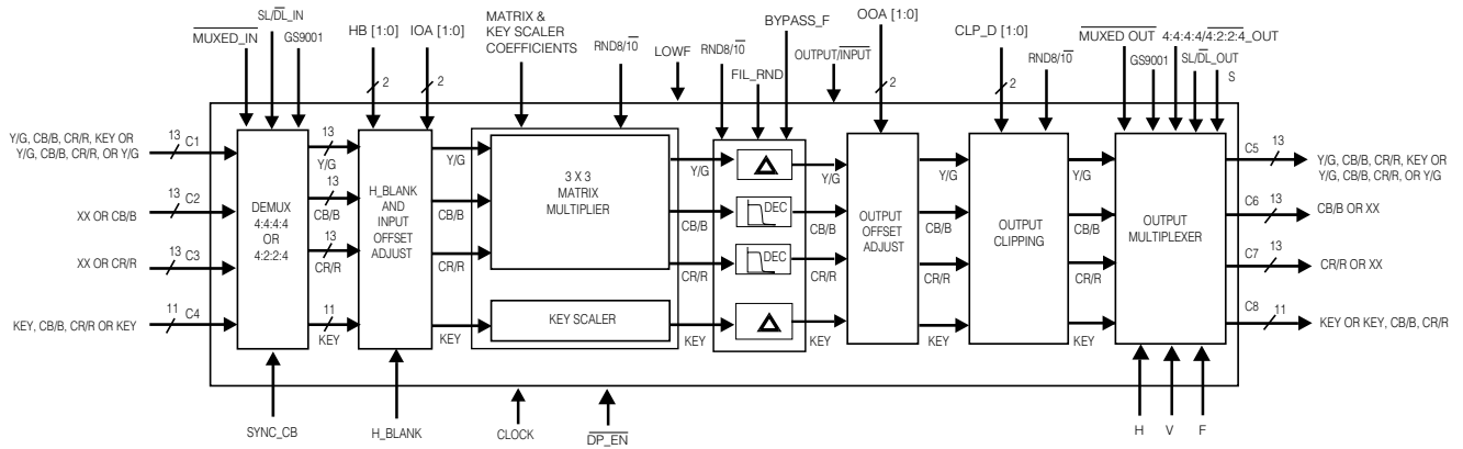
Fig. 5b Functionality of GF9105A Processing Core when \overline{\text{INT/DEC}} = 0 , \text{HV}_F\text{\_OUT} = 0
