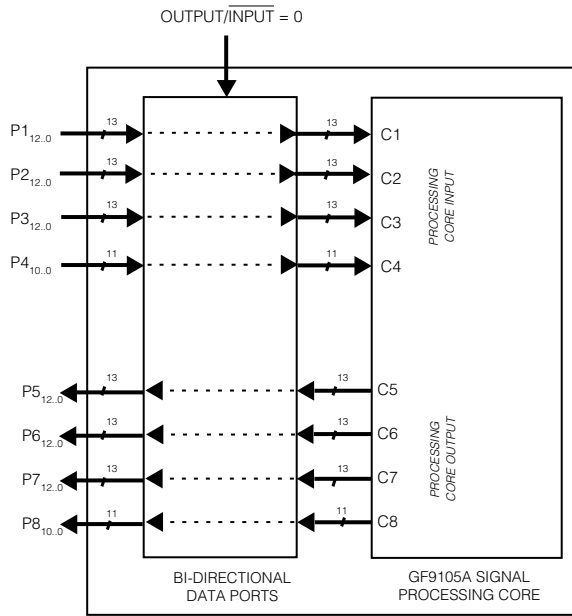
Fig. 4a Functional Block Diagram of GF9105A (OUTPUT/INPUT = 0, HVF_OUT = 0)
