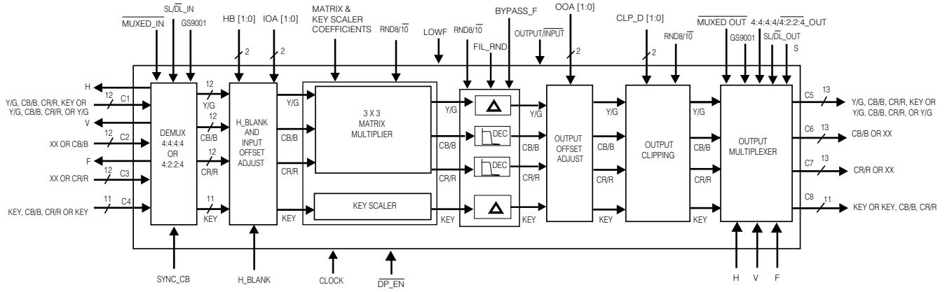
Fig. 5d Functionality of GF9105A Processing Core when \overline{\text{INT/DEC}} = 0 , \text{HVF\_OUT} = 1
