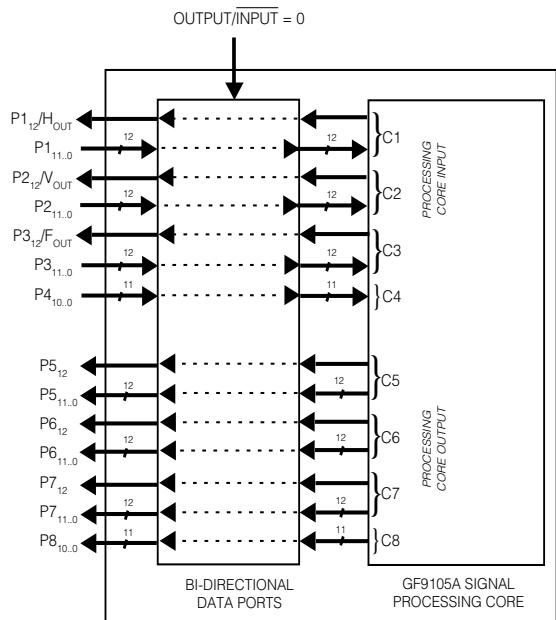
Fig. 4c Functional Block Diagram of GF9105A (OUTPUT/INPUT = 0, HVF_OUT = 1)
