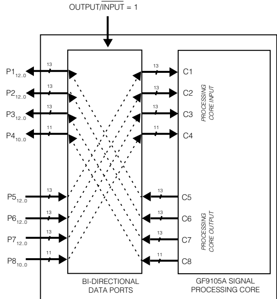
Fig. 4b Functional Block Diagram of GF9105A (OUTPUT/INPUT = 1, HVF_OUT = 0)
