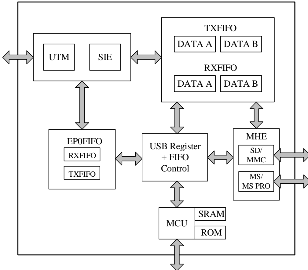
Figure 4.1 - Block Diagram
