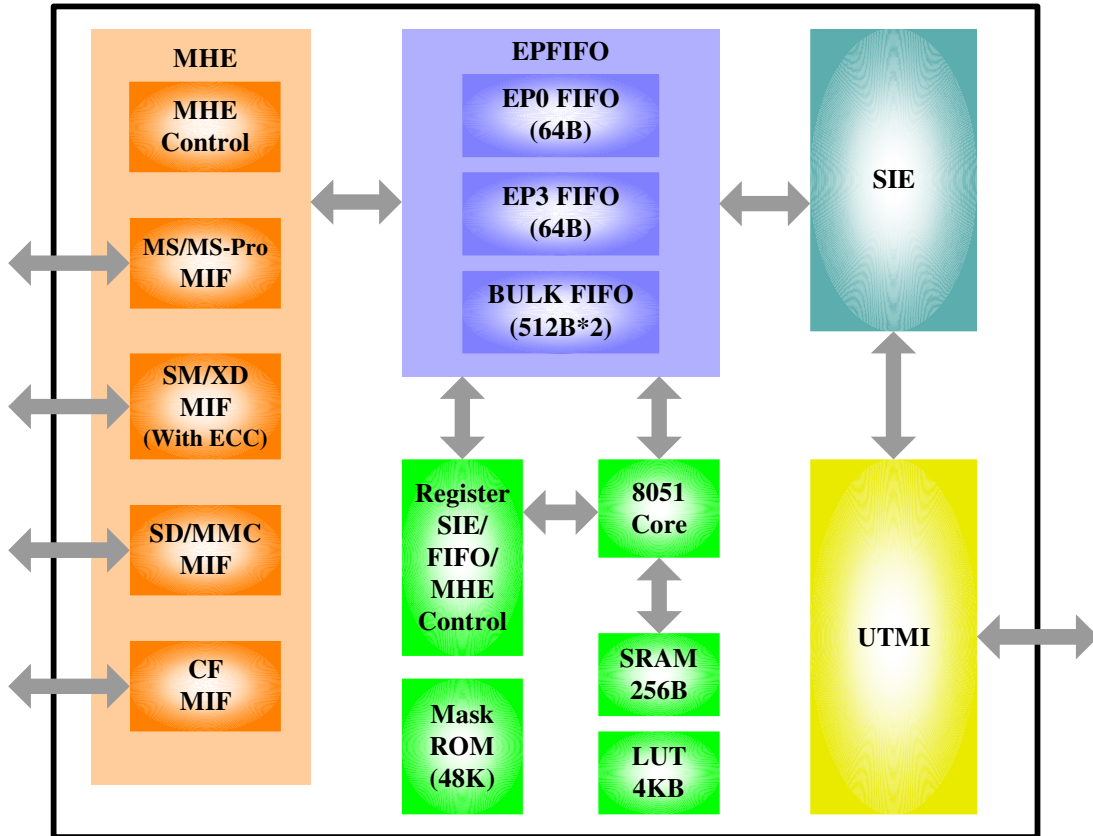
Figure 4.1 - Block Diagram
