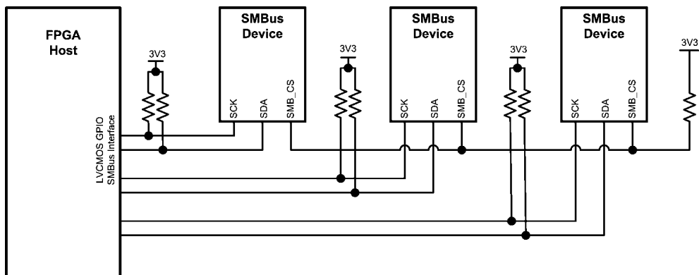
FIGURE 10. SMBus Configuration 3
