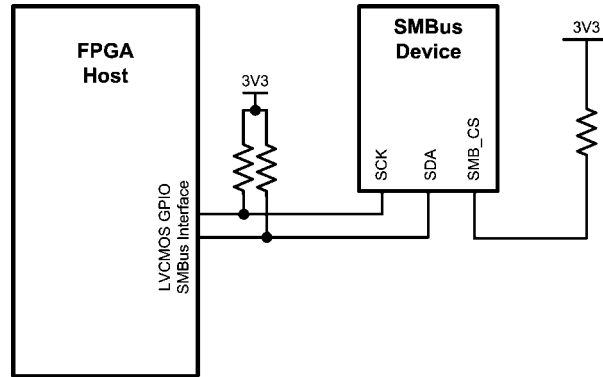
FIGURE 8. SMBus Configuration 1
