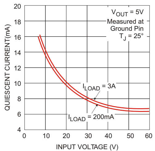
Figure 5. Quiescent Current
