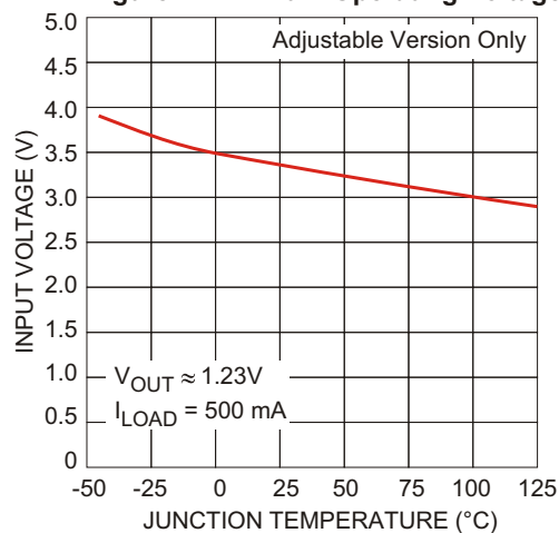
Figure 7. Minimum Operating Voltage
