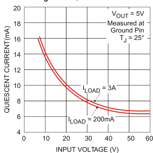
Figure 5. Quiescent Current
