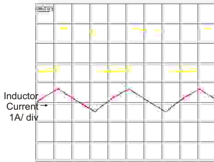
Figure 12. Switching Waveforms
