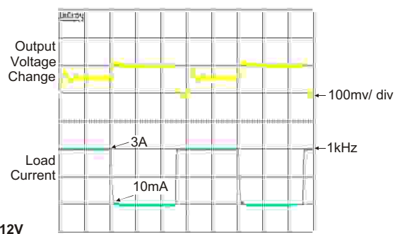
Figure 13. Load Transient Response
