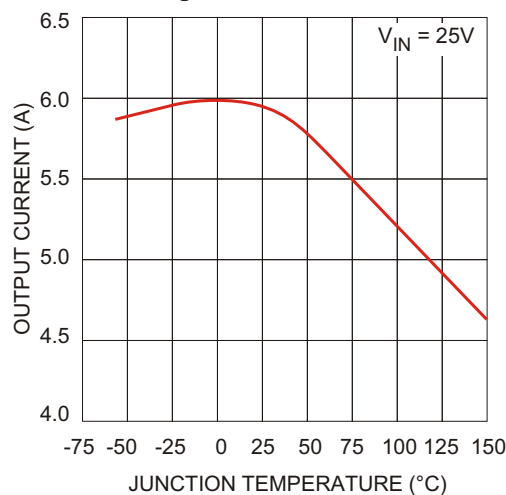
Figure 3. Current Limit
