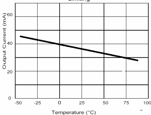
Fig.11 Current Limiting
