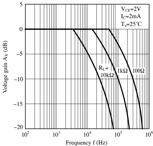
Fig.11 Frequency Response
