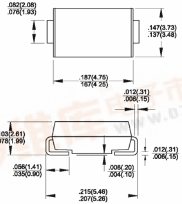
DO-214AA (SMB)
