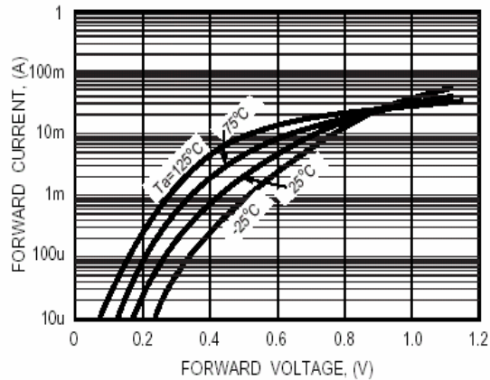
FIG. 1 - FORWARD CHARACTERISTICS
