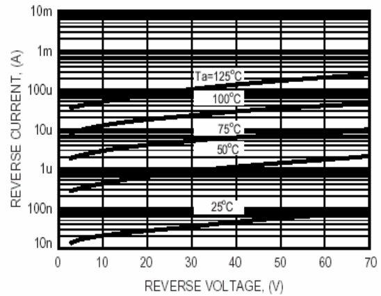
FIG. 2 - REVERSE CHARACTERISTICS
