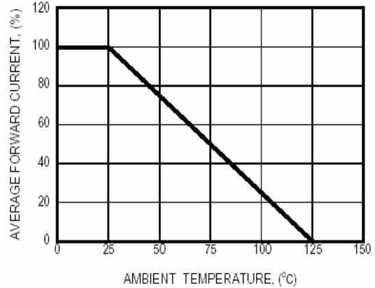
FIG. 4 - TYPICAL FORWARD CURRENT DERATING CURVE
