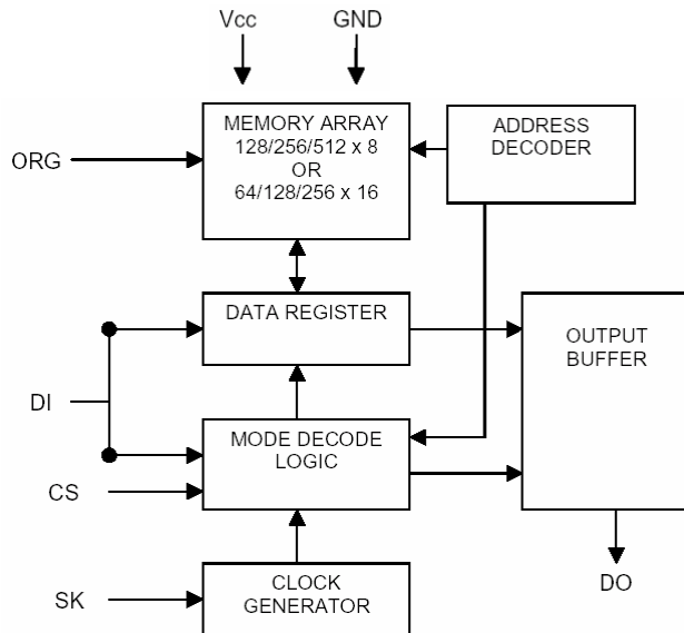
Figure 2. Block Diagram
