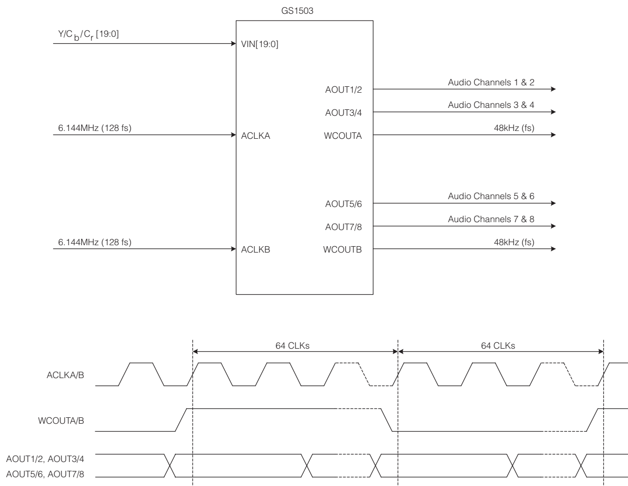
Fig. 38 Serial Audio Output Configuration and Timing
