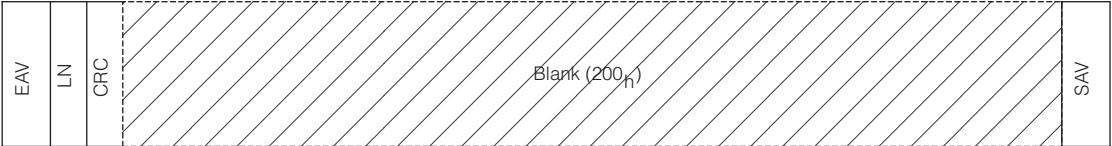
Video Signal before GS1503 (no existing Audio Data Packets)
