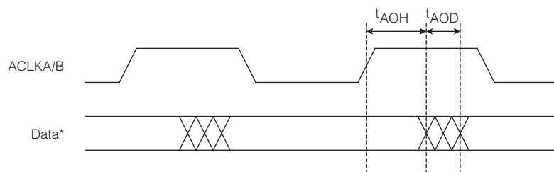
Fig. 4 Audio Data Output Delay & Hold Time
