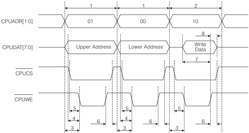
Fig. 8 Host Interface Mode B Write Cycle Timing (CPU_SEL set LOW)
