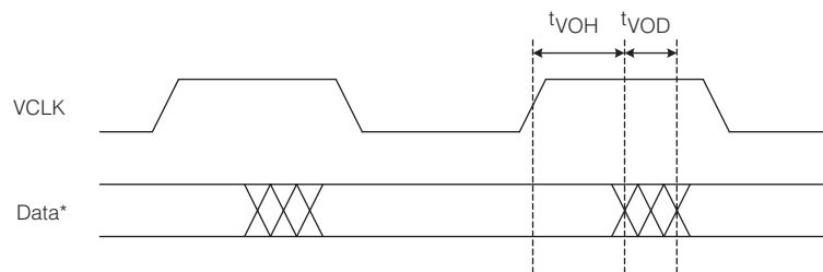
Fig. 2 Video Data Output Delay & Hold Time
