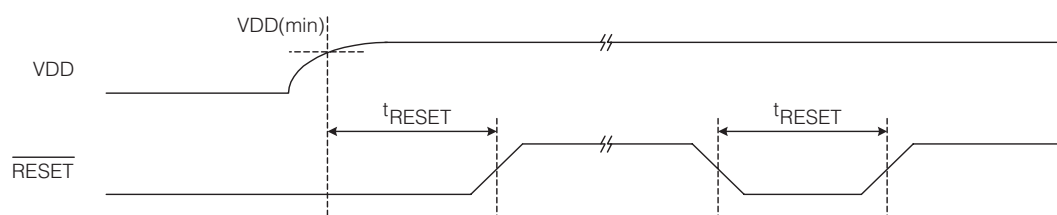
Fig. 5 Reset Timing
