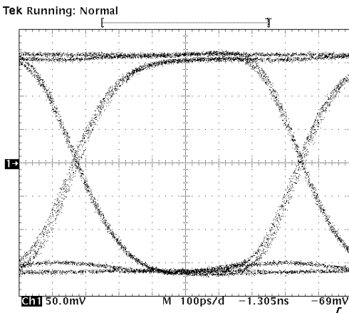
Fig. 3 Output Optimized for Waveform Symmetry L=8.2\text{nH} , R=75 (Typical ORL=13.5dB)
