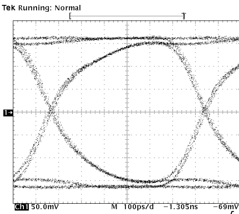
Fig. 4 Output Optimized for Return Loss L=12\text{nH} , C=0.5\text{pF} , R=75 (Typical ORL=18dB)
