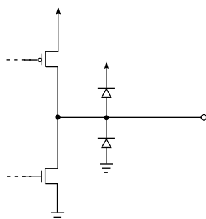
Figure 3-7: Indicator Outputs: \overline{SD/HD} , LOCKED, LOS
