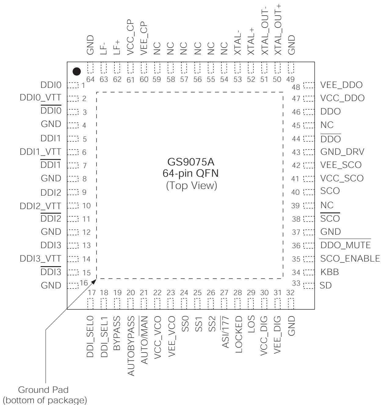
Figure 1-2: 64-Pin QFN
