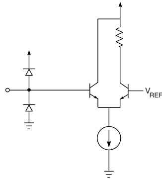
Figure 3-1: TTL Inputs
