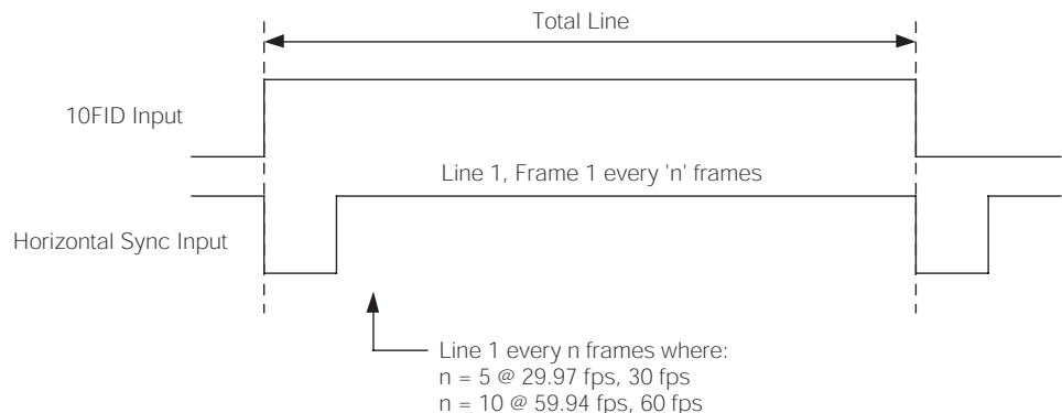
Figure 3-5: 10FID Input Timing
