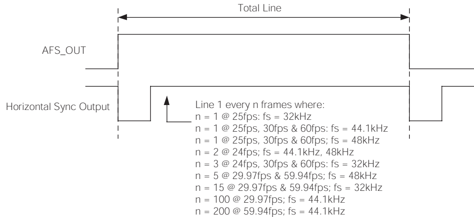
Figure 3-10: AFS Output Timing
