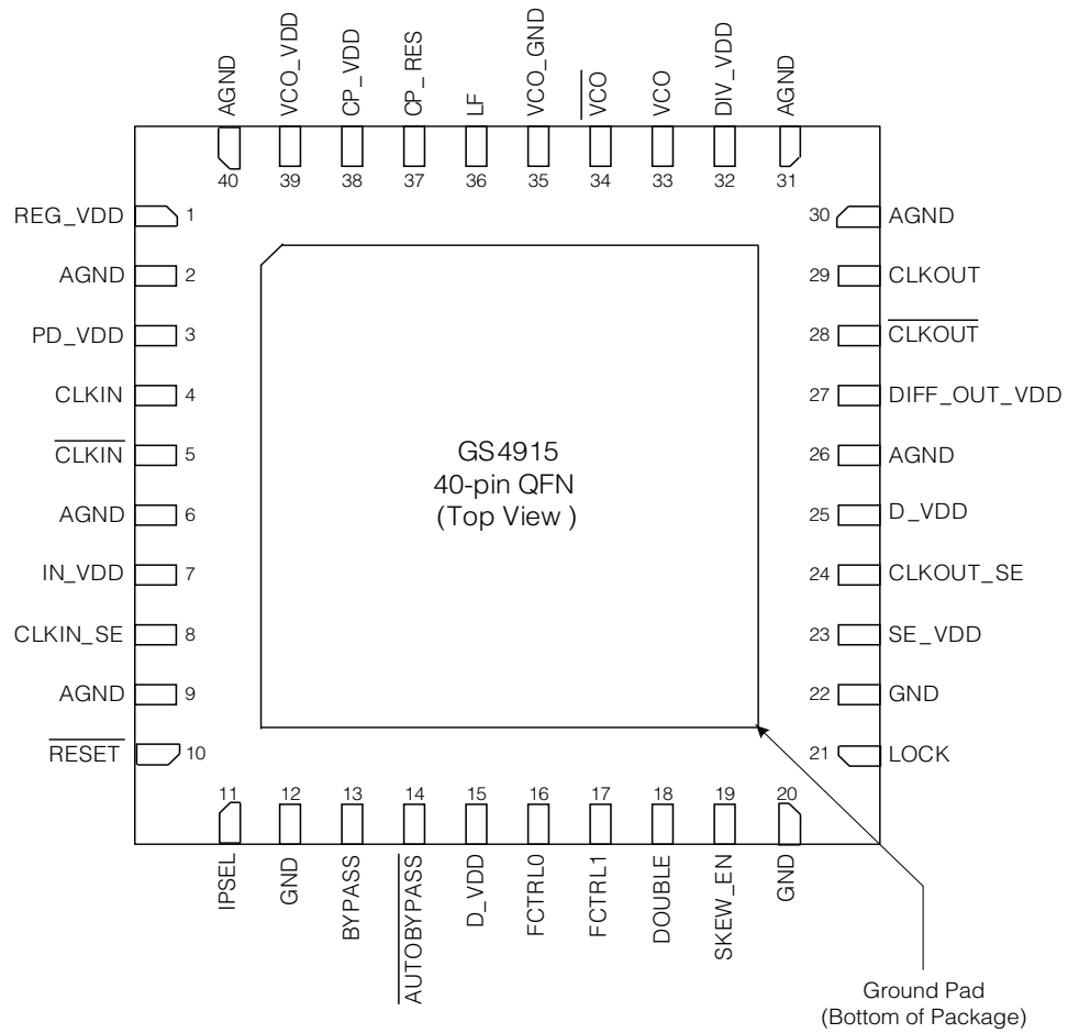
Figure 1-1: 40-Pin QFN
