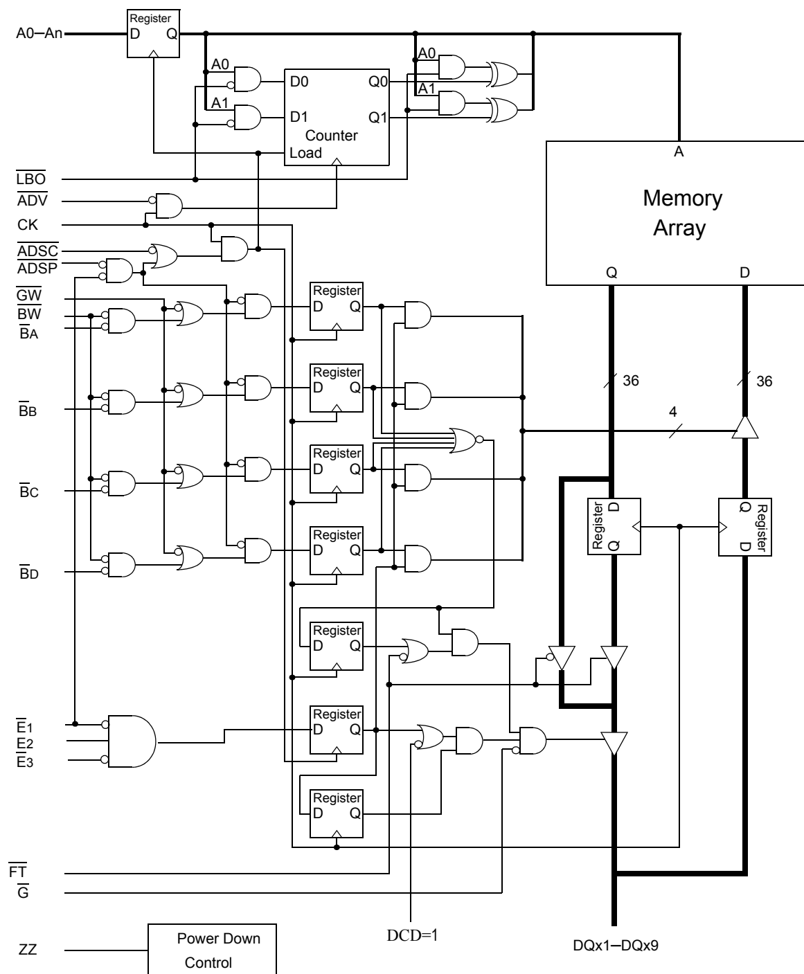
GS8640E18/32/36-xxxV Block Diagram
