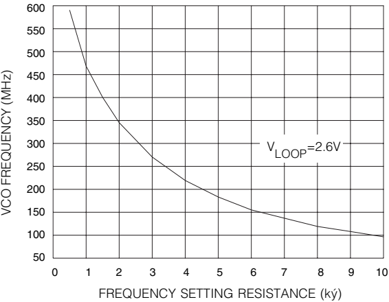
Fig. 12 VCO Frequency
