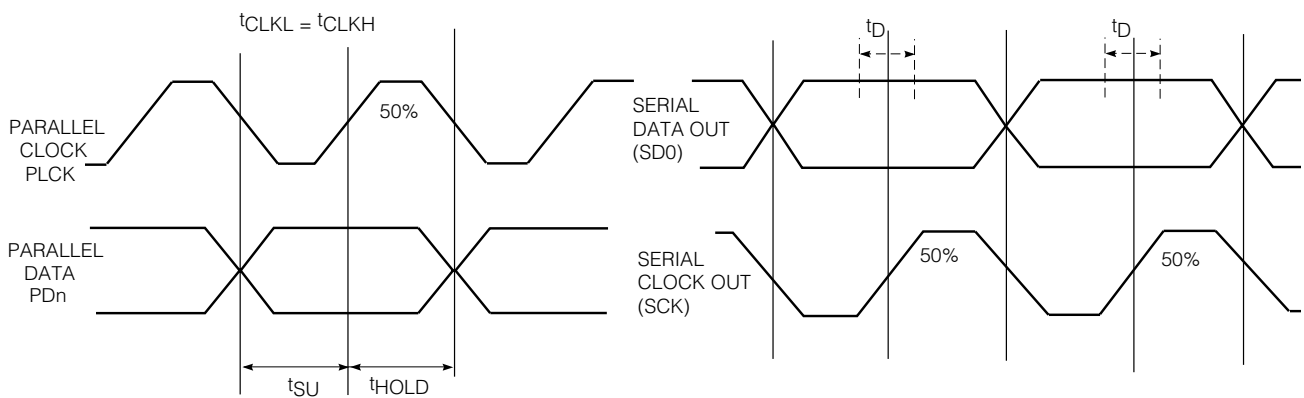
Fig. 9 Waveforms
