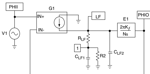
Fig. 16 SPICE Model of PLL
