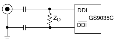
Fig. 19 Recommended Interface for Single-Ended Driver
