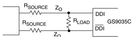
Fig. 18 Recommended Interface for Differential Signals
