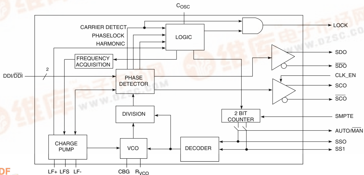
BLOCK DIAGRAM
