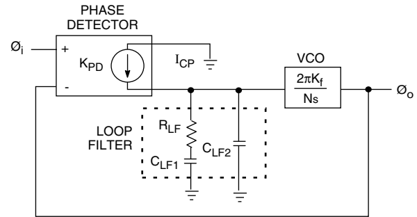
Fig. 13 PLL Model
