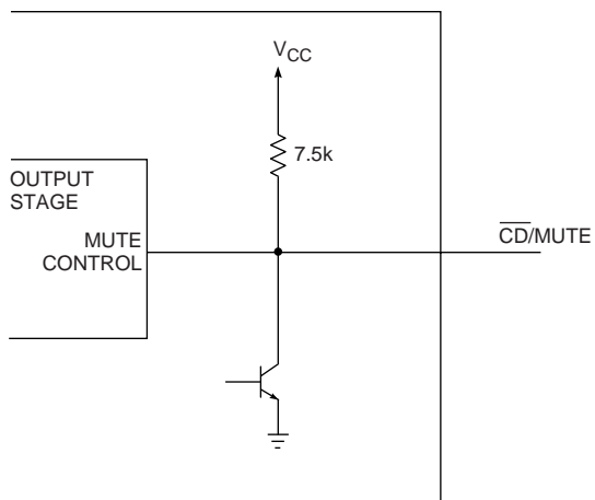
Figure 3 \overline{\text{CD}}/\text{MUTE} Circuit
