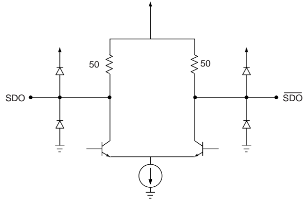
Figure 4 Output Circuit
