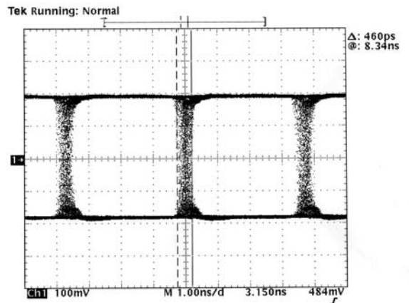
Figure 12 Output 8281, 280m, 270Mb/s
