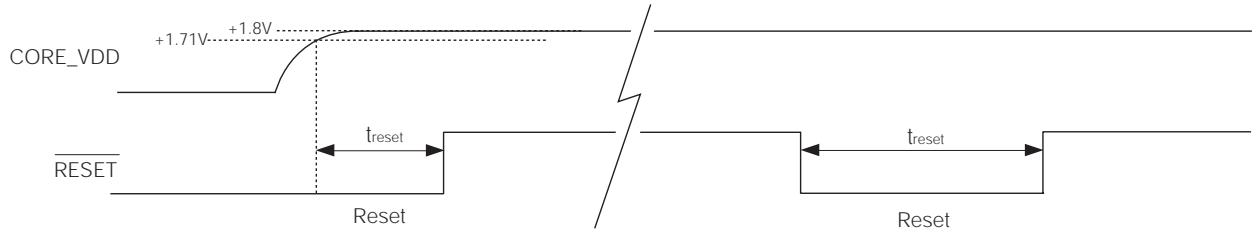
Figure 3-23: Reset pulse
