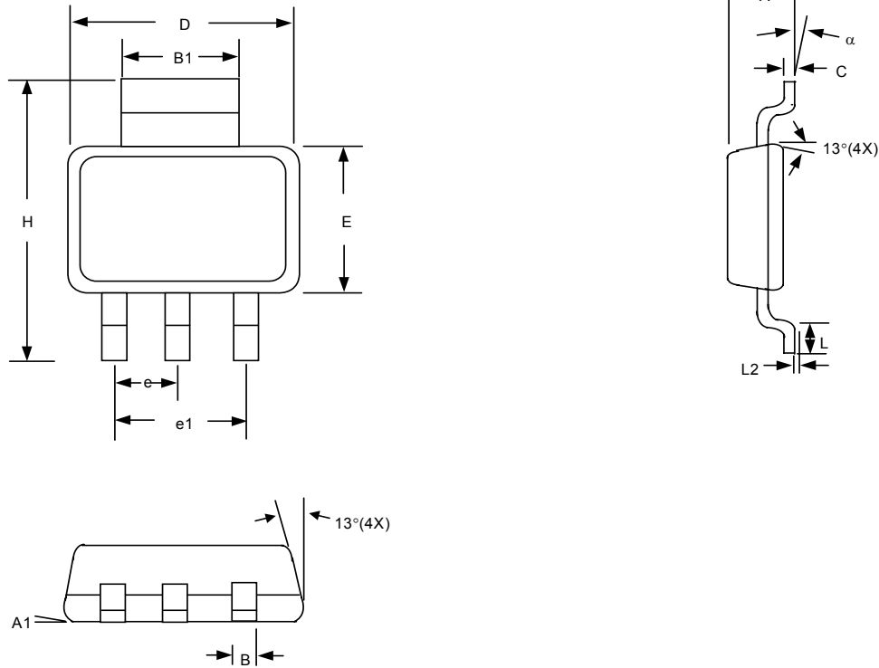
SOT-223 (T6) Package
