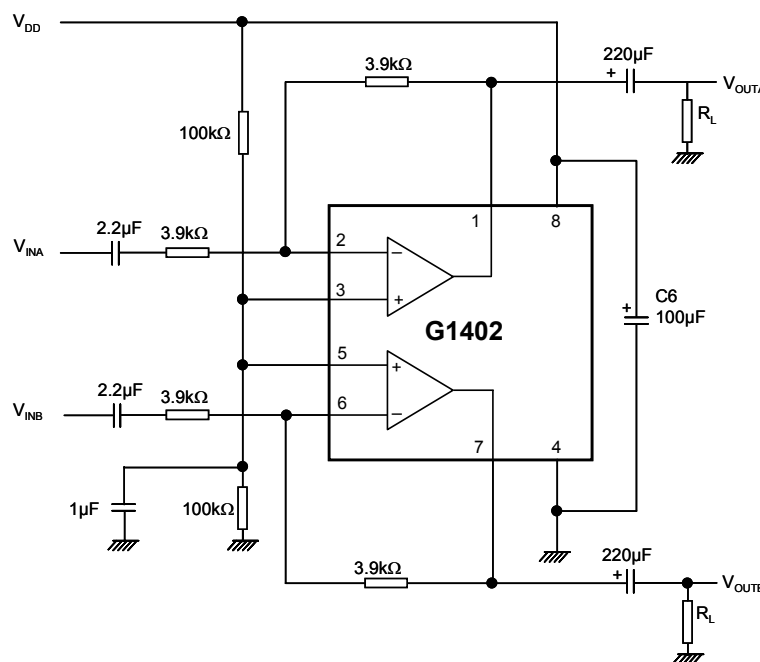
Fig.1 Measurement circuit for inverting application
