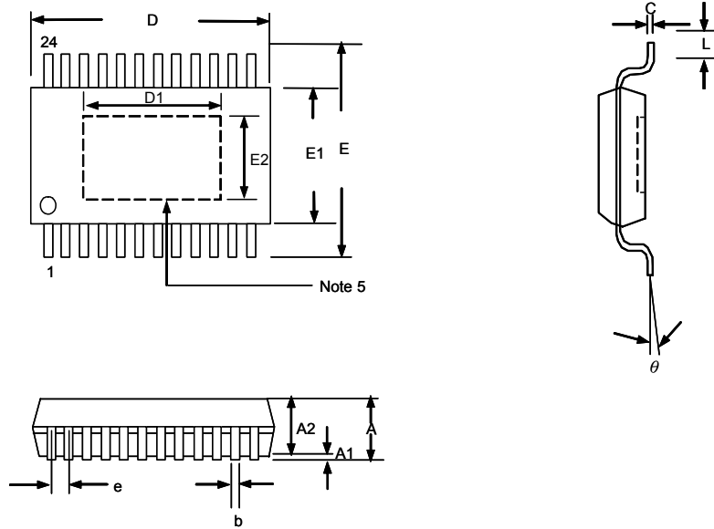
TSSOP-24 (FD) Package
