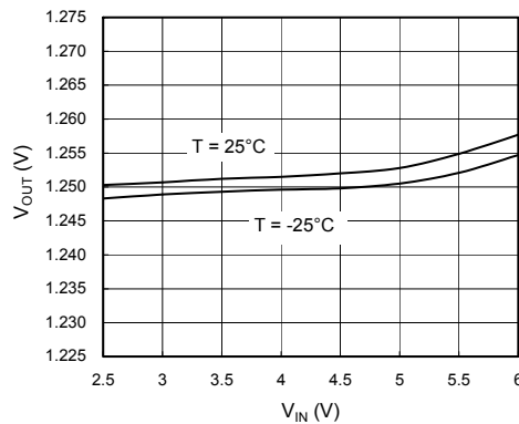
Line Regulation
