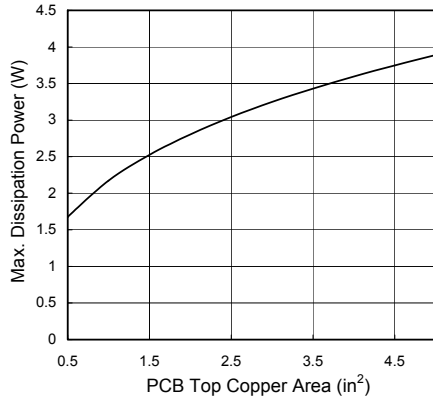
G1084T53(TO-263) Max. Power Dissipation vs. PCB Top Copper Area Area T_{AMB} = 25^{\circ}\text{C} ; Still Air
