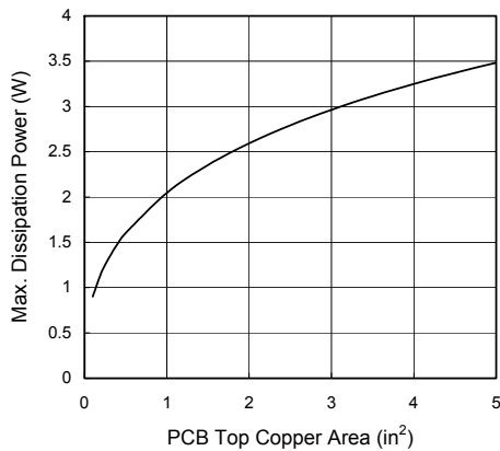
G1084T43(TO-252) Max. Power Dissipation vs. PCB Top Copper Area Area T_{AMB} = 25^{\circ}\text{C} ; Still Air
