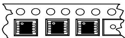
Feed Direction Typical SOP Package Orientation
