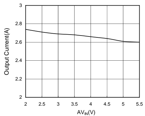
Maximum Sourcing Current vs AV_{IN} ( V_{DDQ}=1.8V , PV_{IN}=3.3V )
