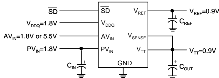
Figure 5. Recommended DDR-II Termination
