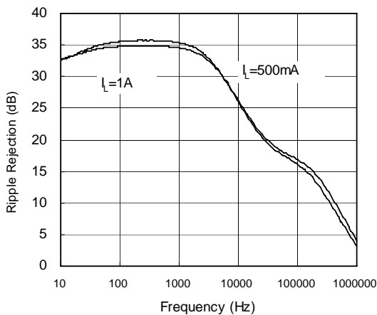
Ripple Rejection
