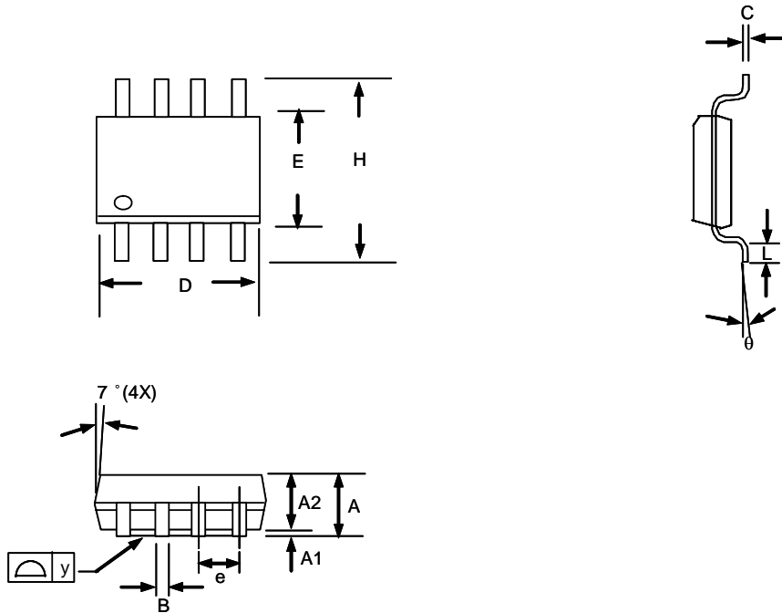
SOP-8 Package
