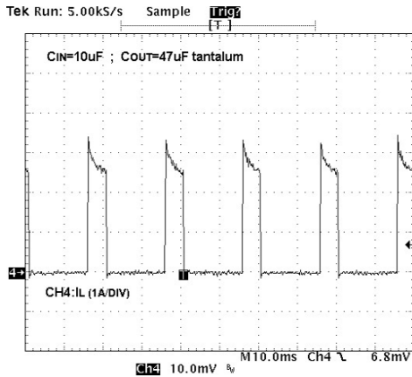
Short Circuit-Current
