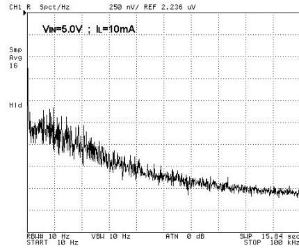
Output Noise
