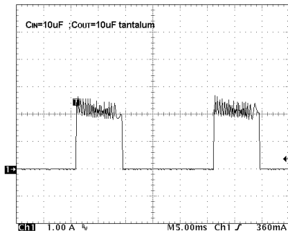
Short Circuit-Current
