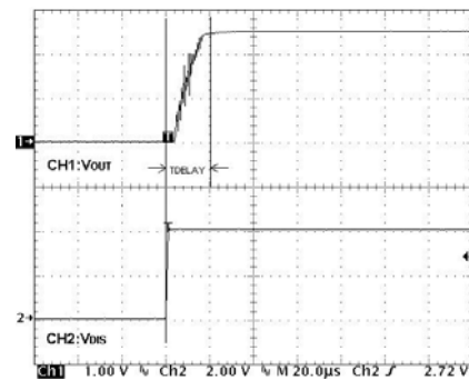
Disable- ON
