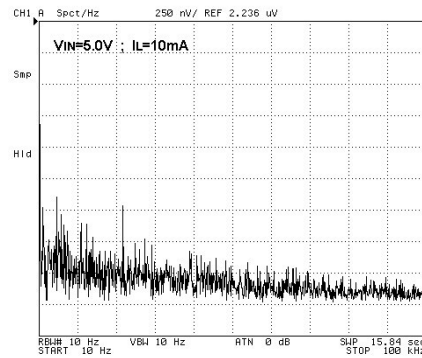
Output Noise
