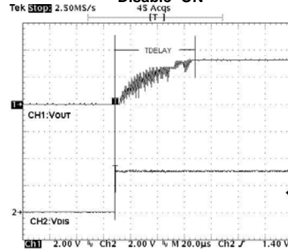
Disable- ON
