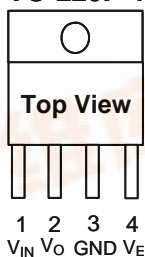
TO-220F-4
