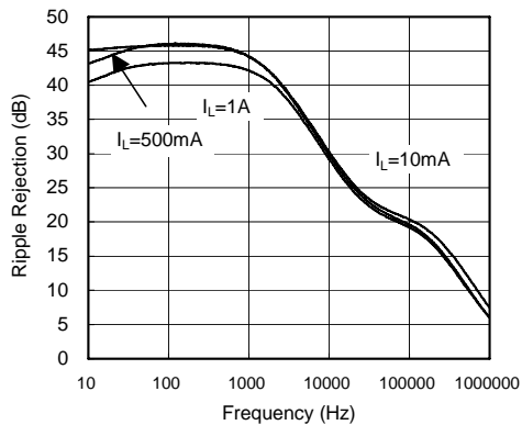
Ripple Rejection
